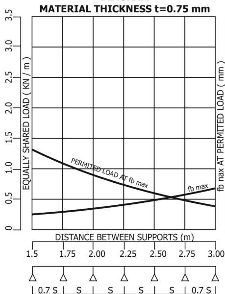
CABLE TRAY H:110 LOADING DIAGRAM
