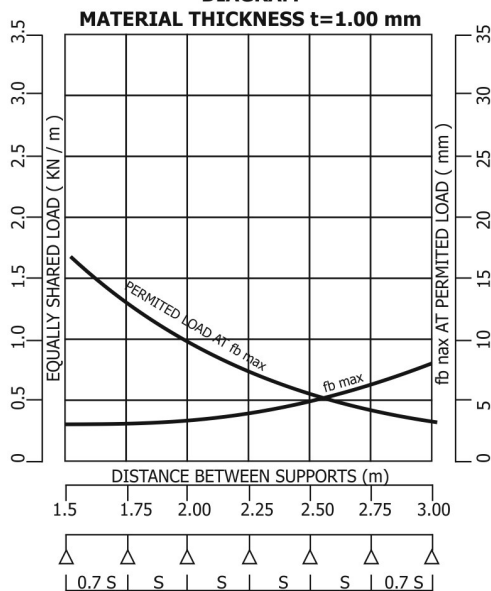
CABLE TRAY H:85 LOADING DIAGRAM
