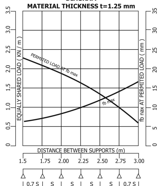
CABLE TRAY H:85 LOADING DIAGRAM
